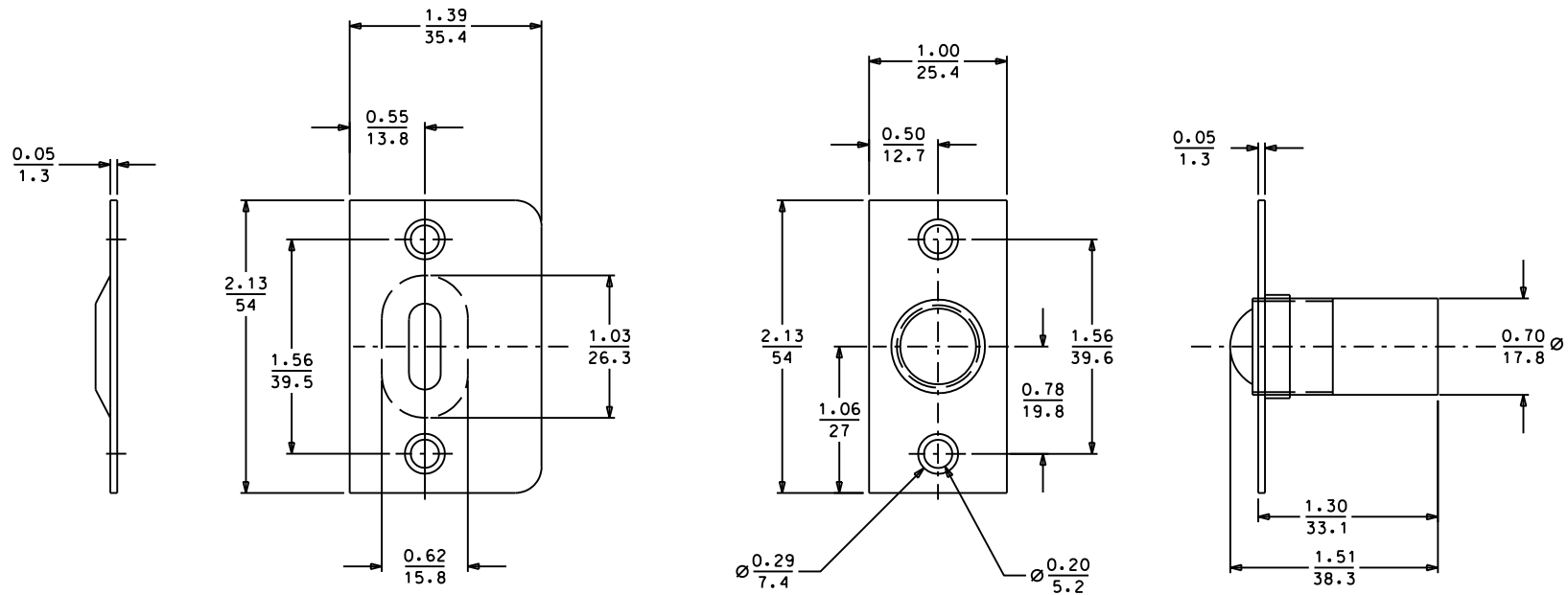
BALL LATCH
